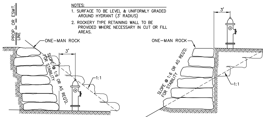
FIRE HYDRANT IN CUT
